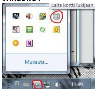
Windows 7
