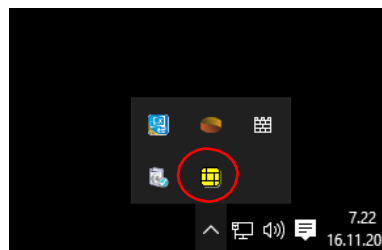
Windows 10
